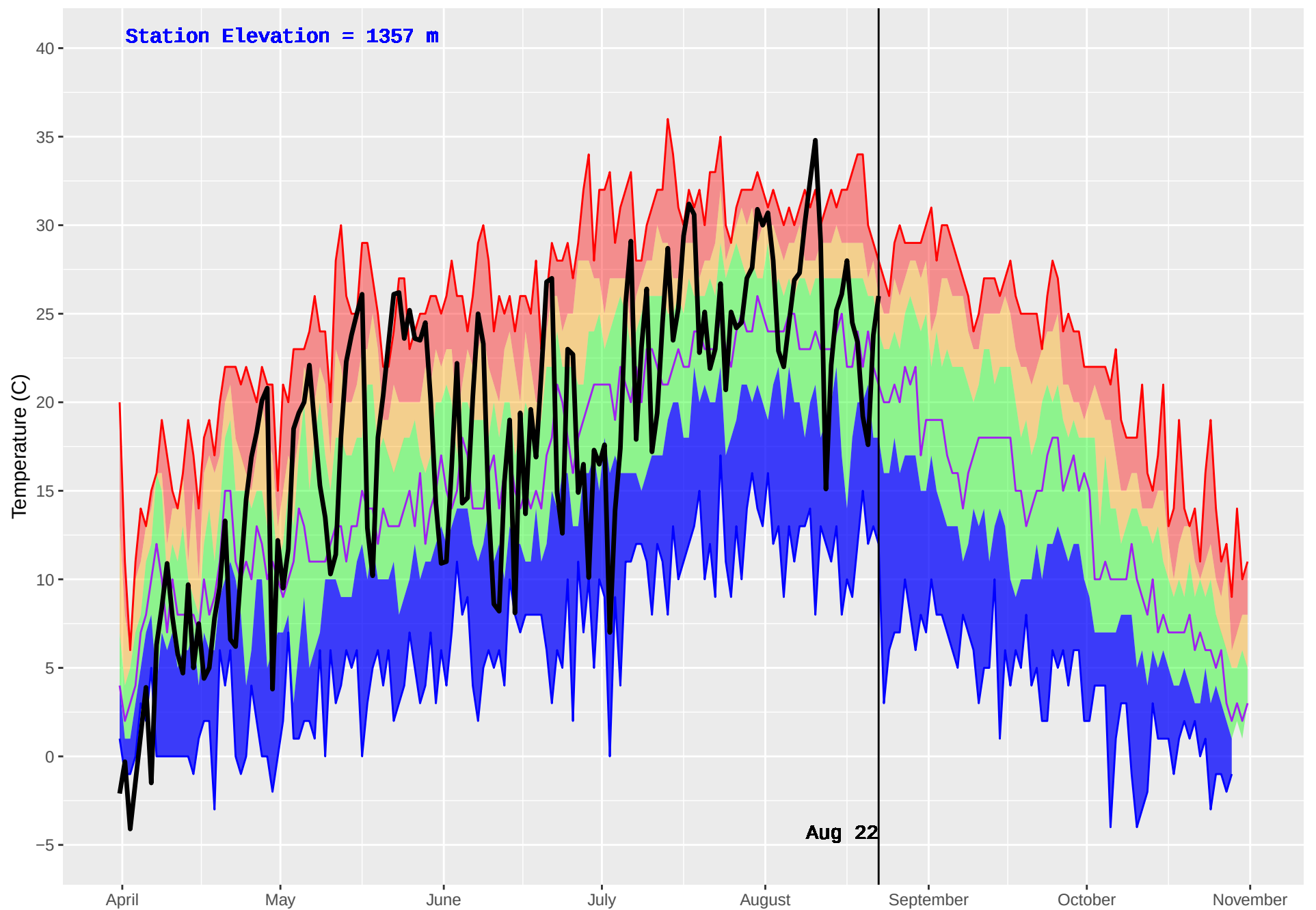
WHITE RIVER (790) : Historical (1989–2016) and Current (2018) Daily Temperature
