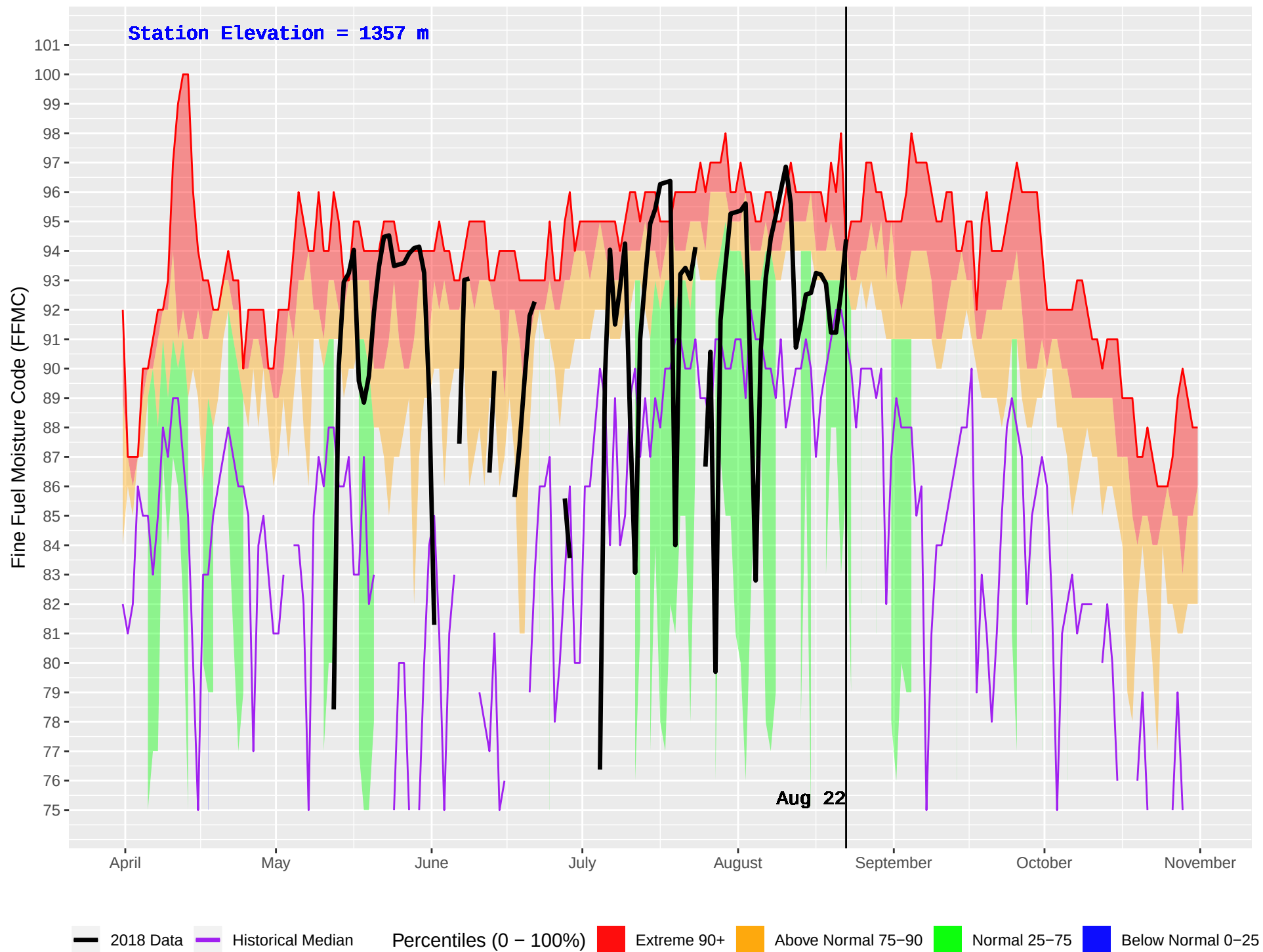
WHITE RIVER (790) : Historical (1989–2016) and Current (2018) Daily Fine Fuel Moisture Code (FFMC)
