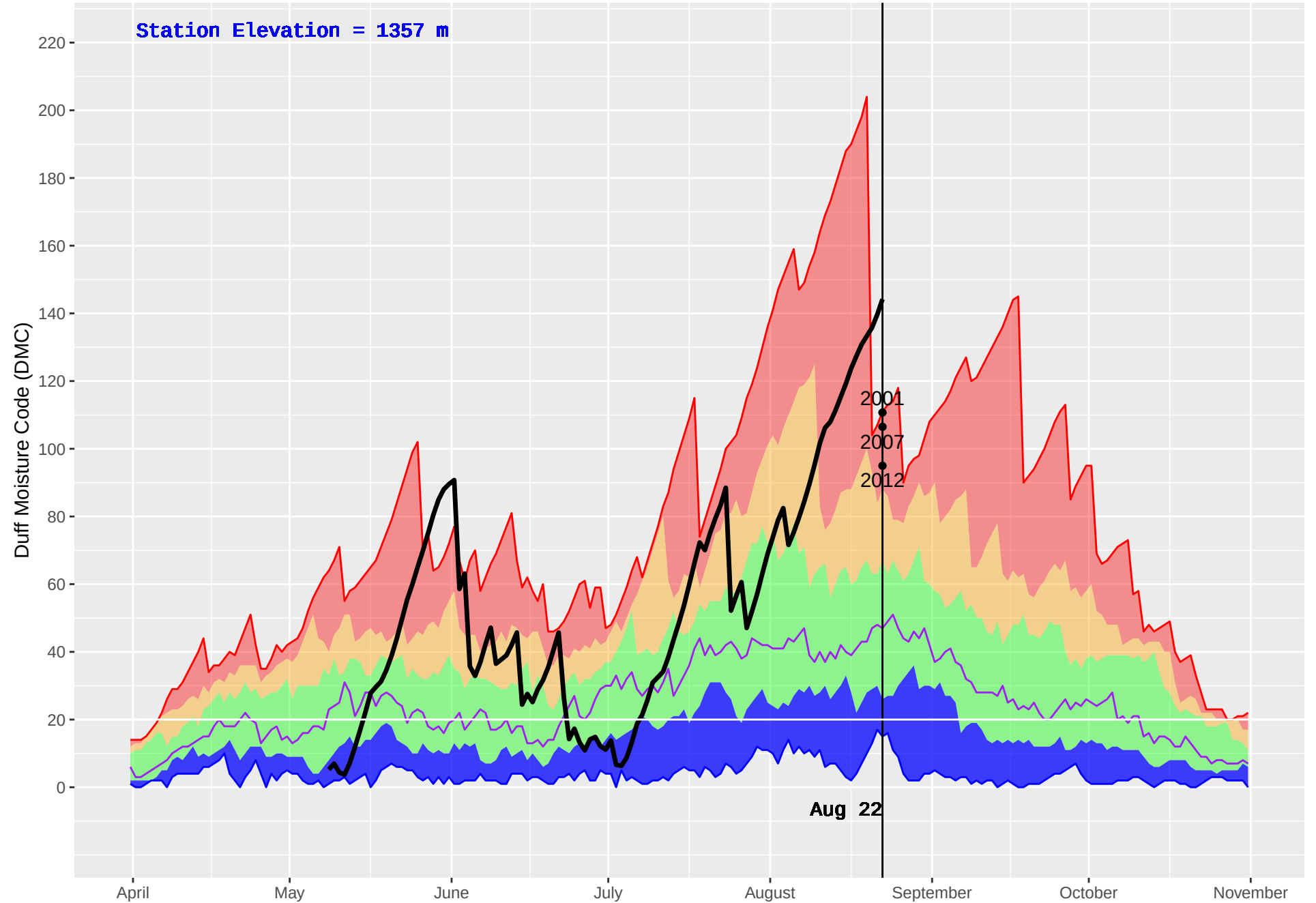
WHITE RIVER (790) : Historical (1989–2016) and Current (2018) Daily Duff Moisture Code (DMC)
