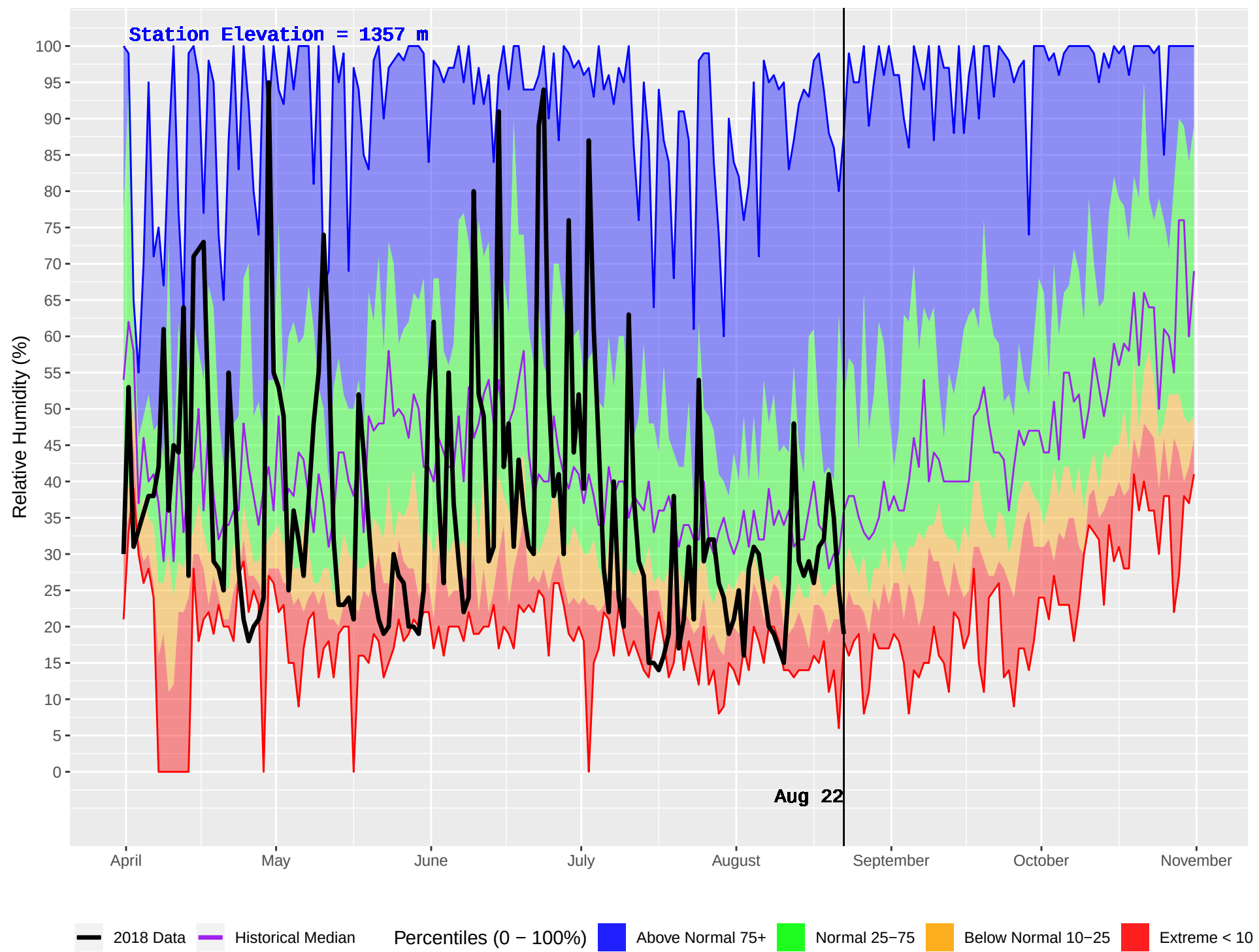
WHITE RIVER (790) : Historical (1989–2016) and Current (2018) Daily Relative Humidity
