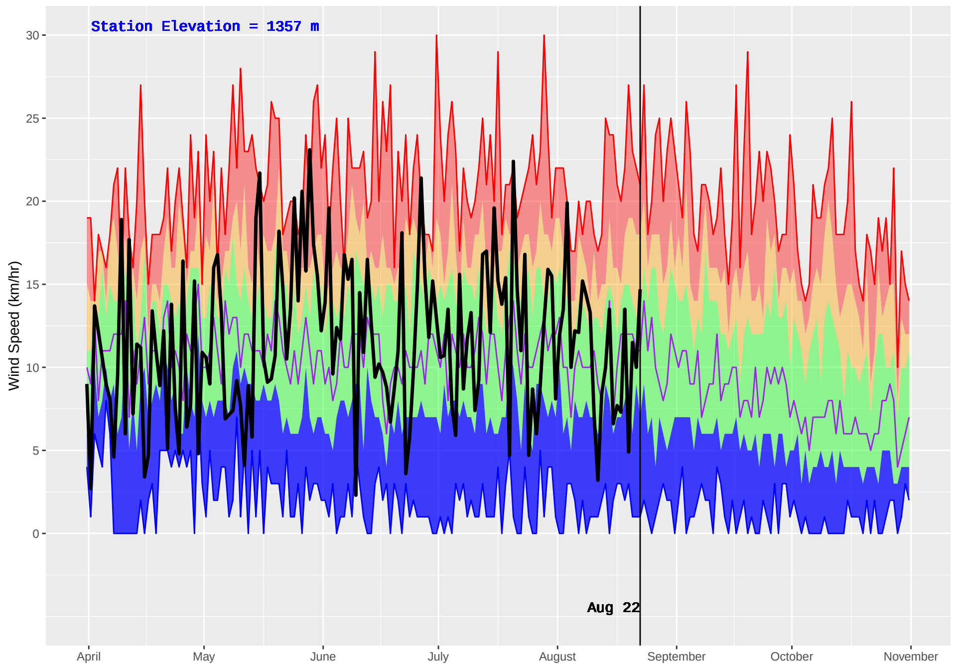
WHITE RIVER (790) : Historical (1989–2016) and Current (2018) Daily Wind Speed
