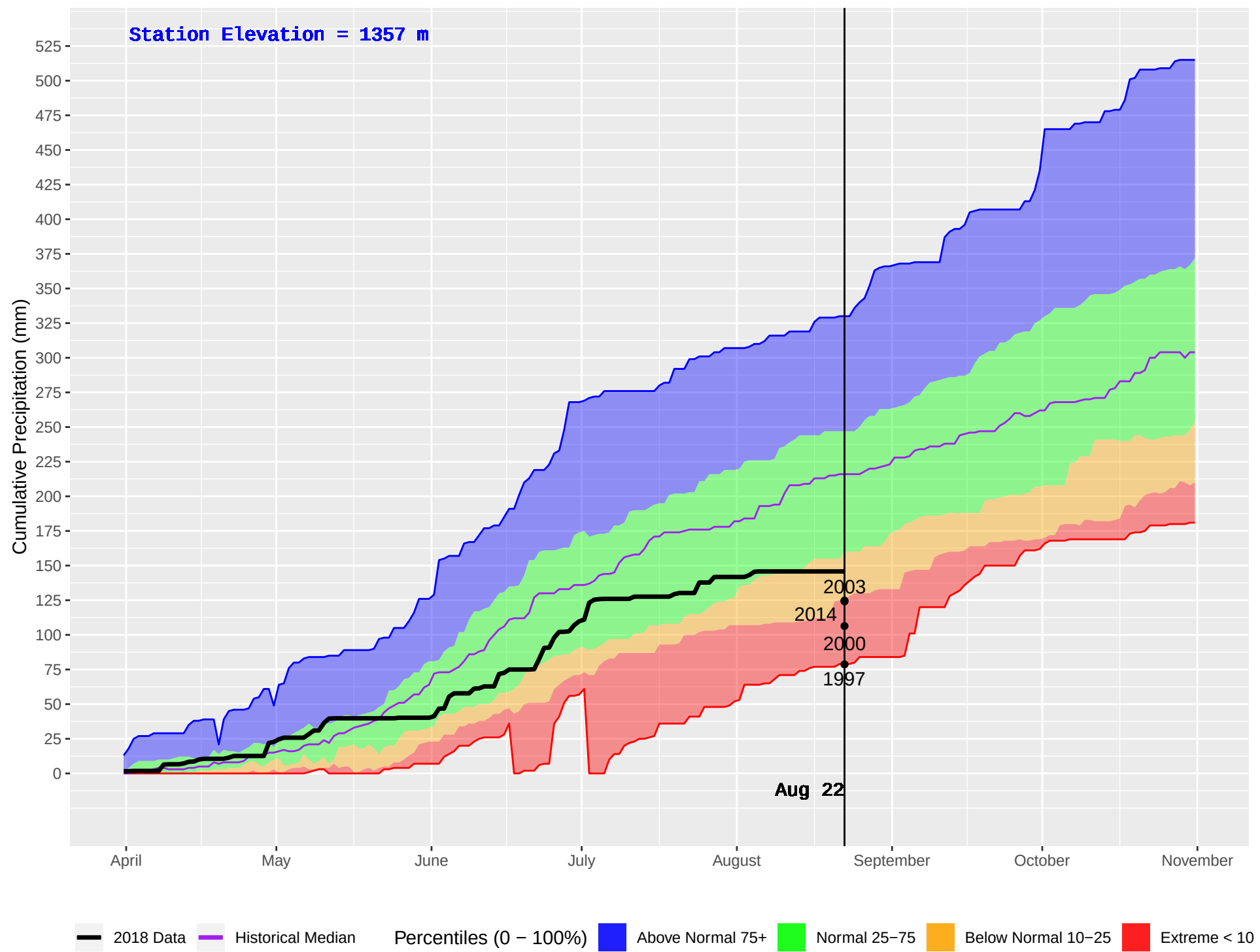
WHITE RIVER (790) : Historical (1989–2016) and Current (2018) Daily Cumulative Precipitation
